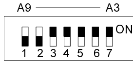
Figure 2: DIP-switch Illustration
