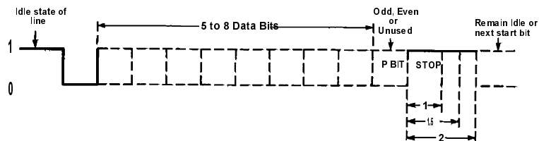
Figure 13: Asynchronous Communications Bit Diagram
