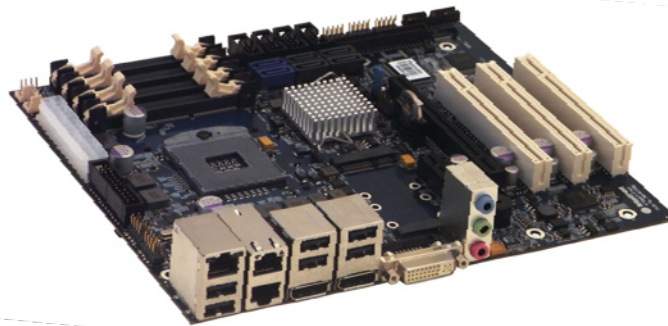
KTQM67/Flex
