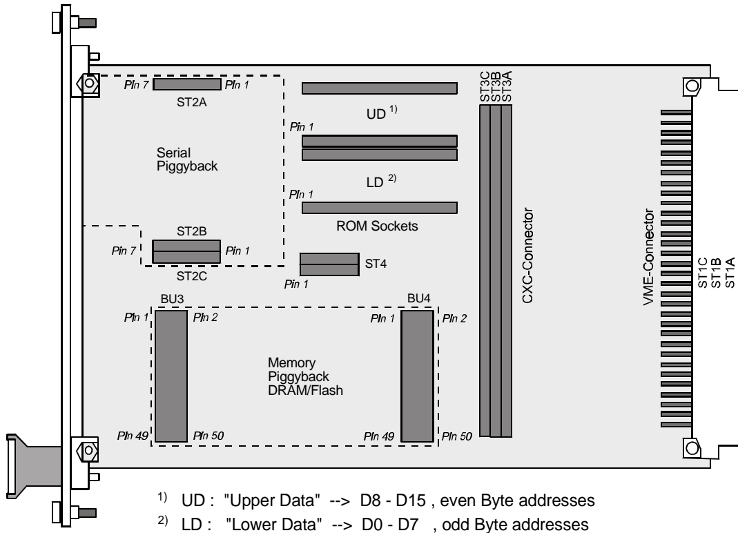
Figure 4.1.0.1: Main Board Connector Overview
